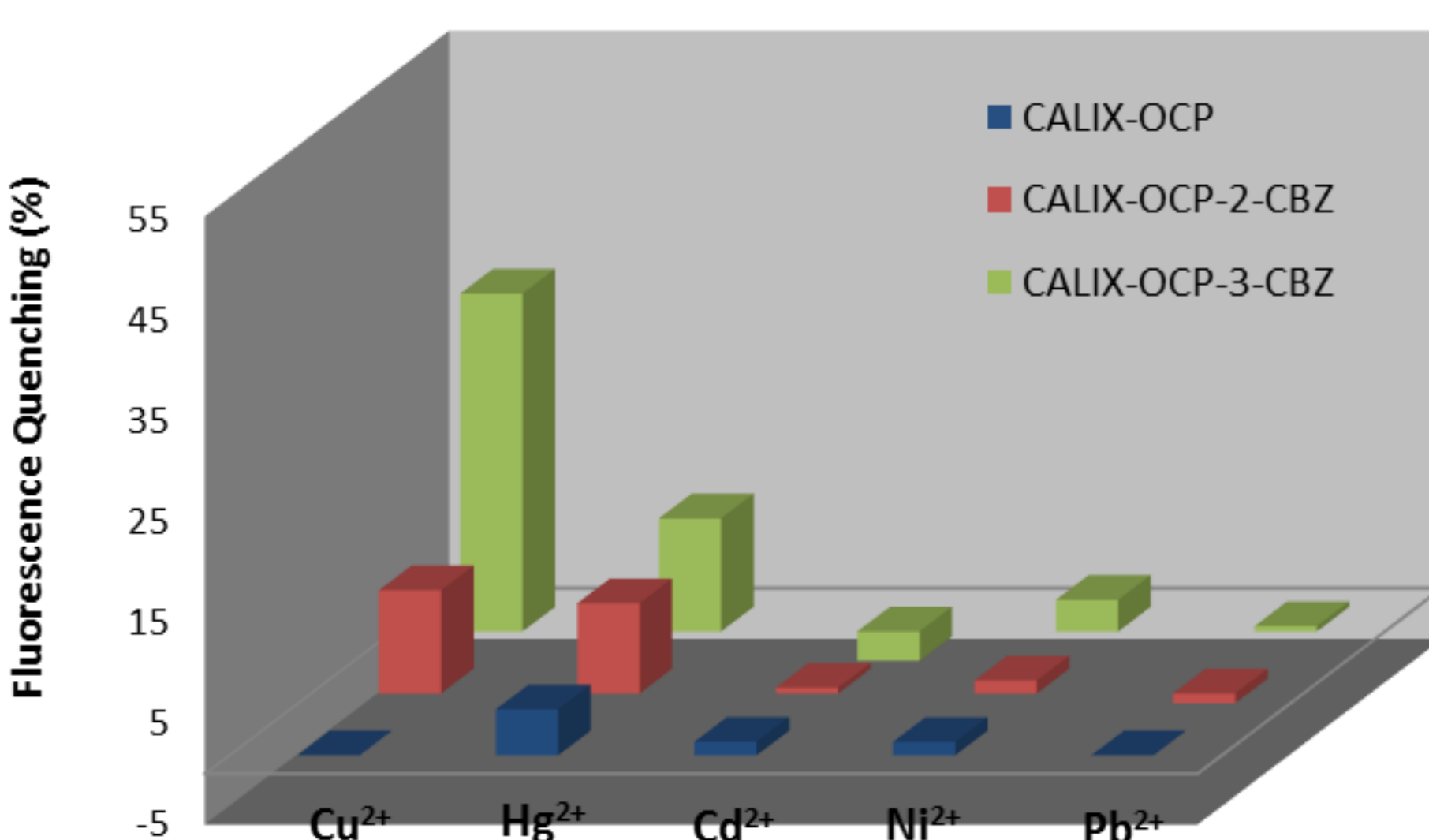
Fig. 2. Comparative fluorescence quenching of several fluorophores ( 1.0 \times 10^{-7} M in CH 3 CN) towards different metal cations (33 eq.).
