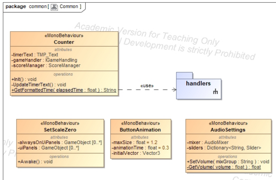
Figure 4.5: Common Package UML
