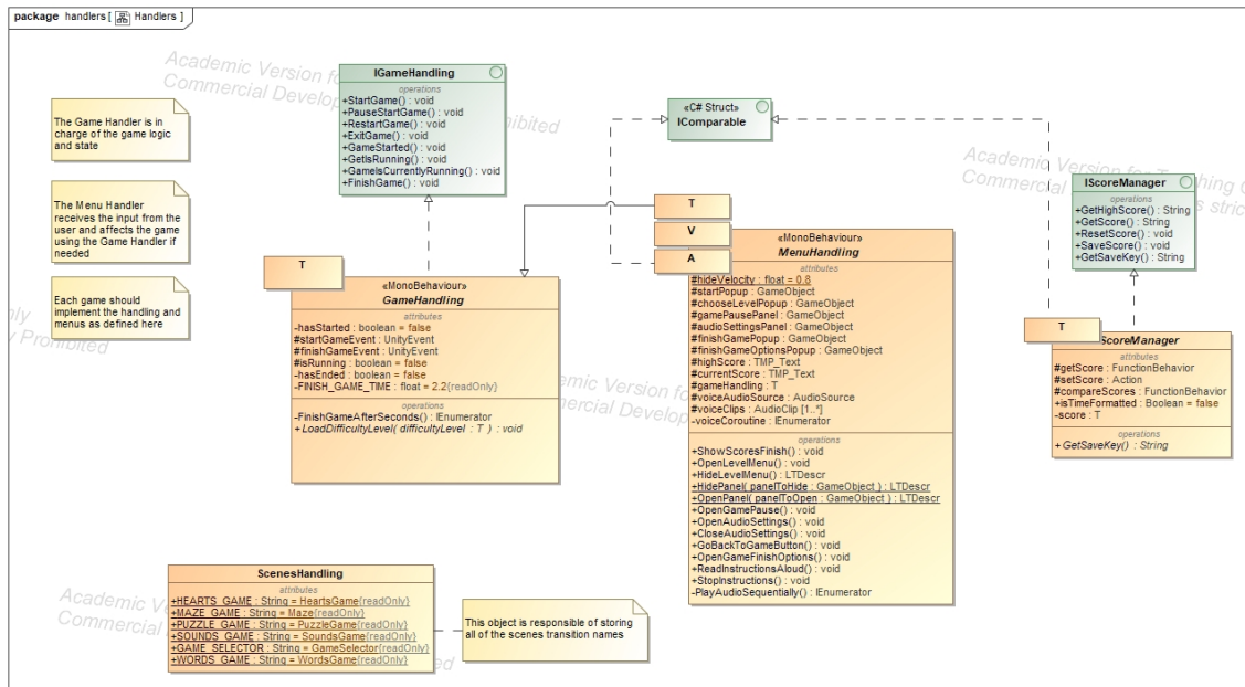
Figure 4.4: Handlers Mechanism UML
