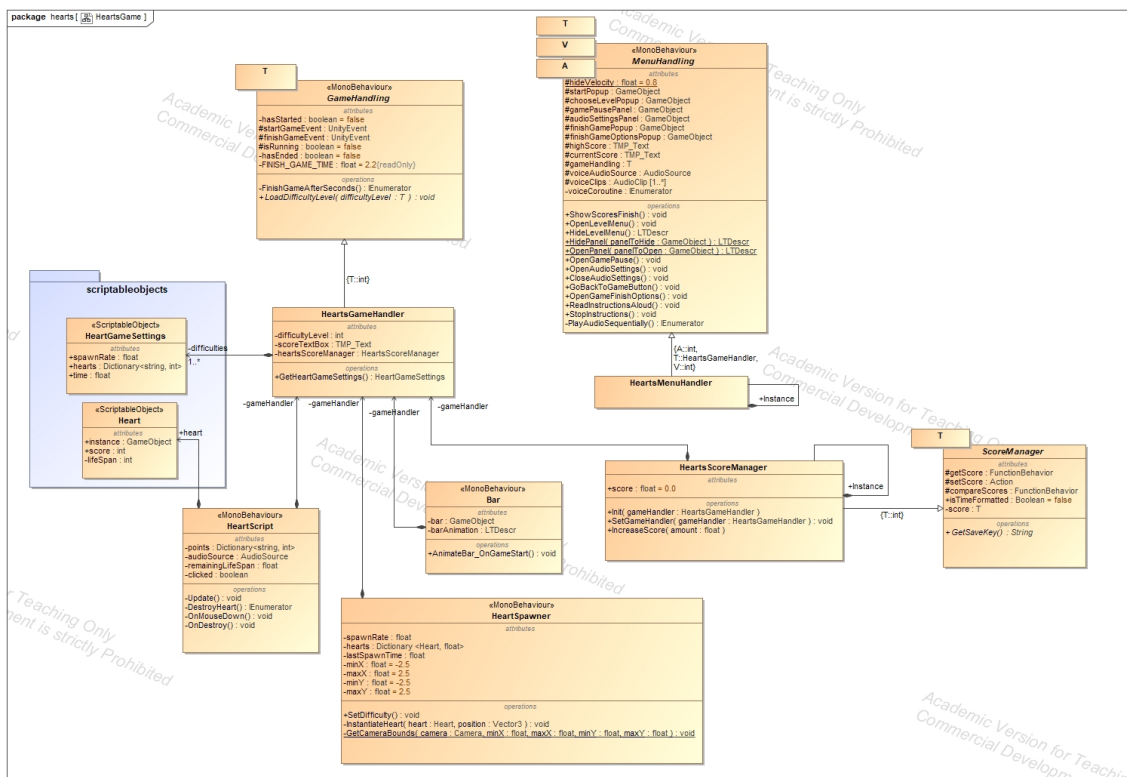
Figure 4.6: Hearts Game entities - UML
