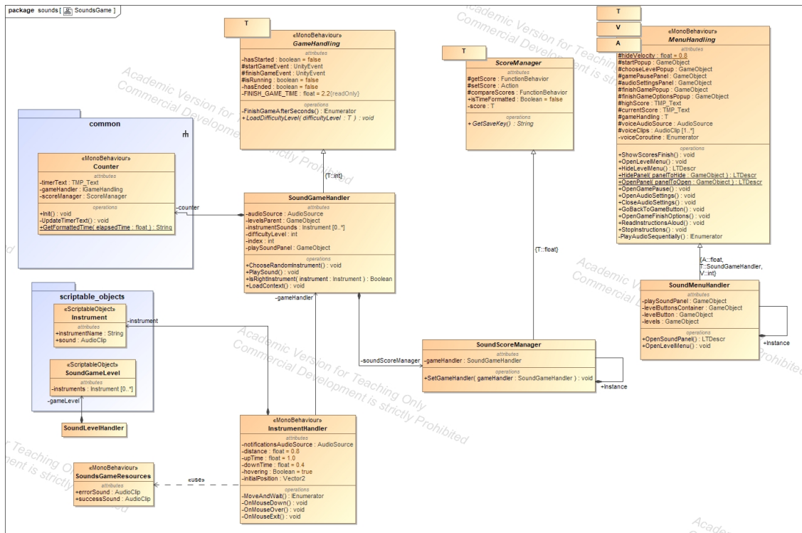
Figure 4.8: Sounds Game Entities - UML
