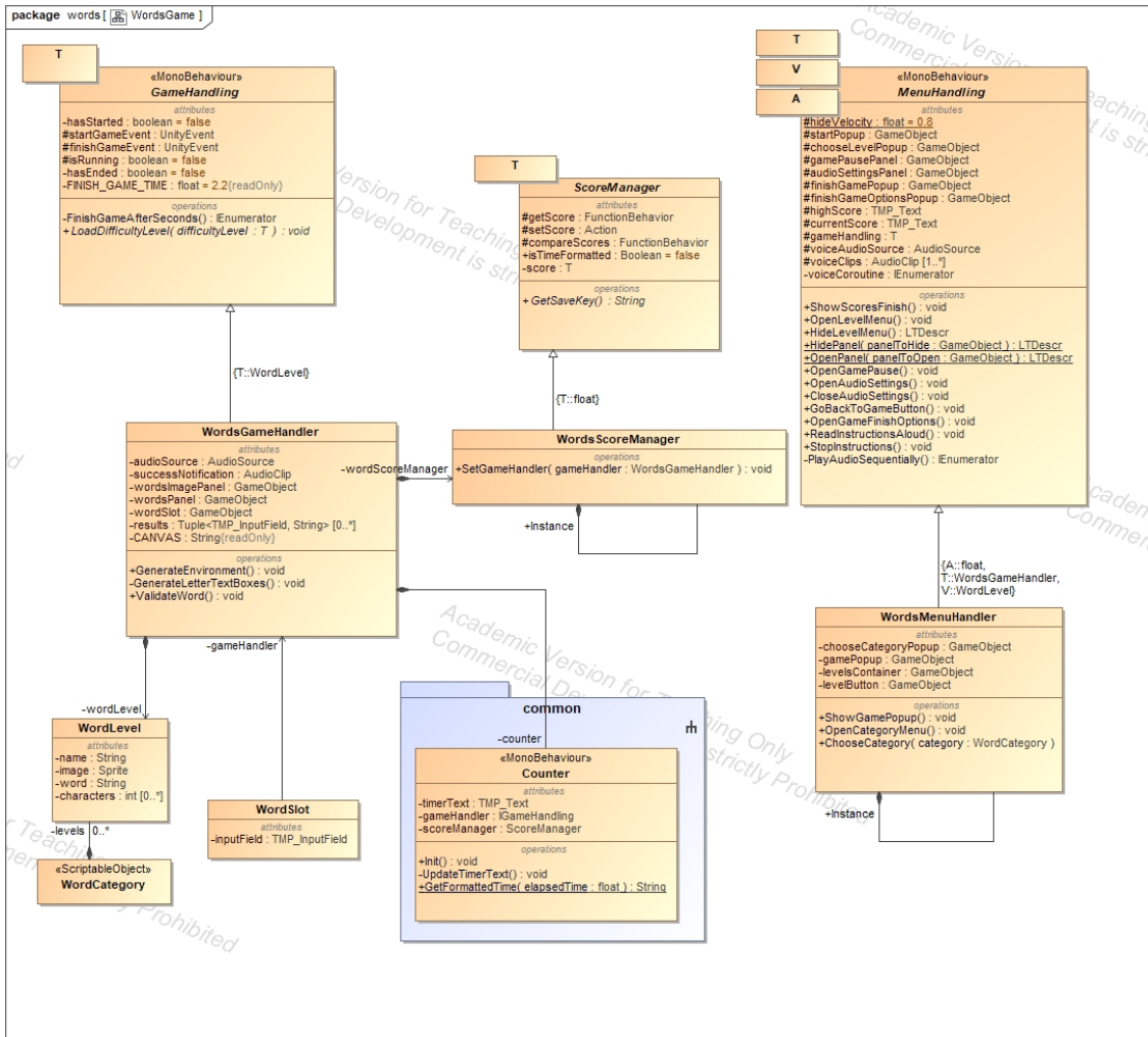
Figure 4.9: Words Game Entities - UML
