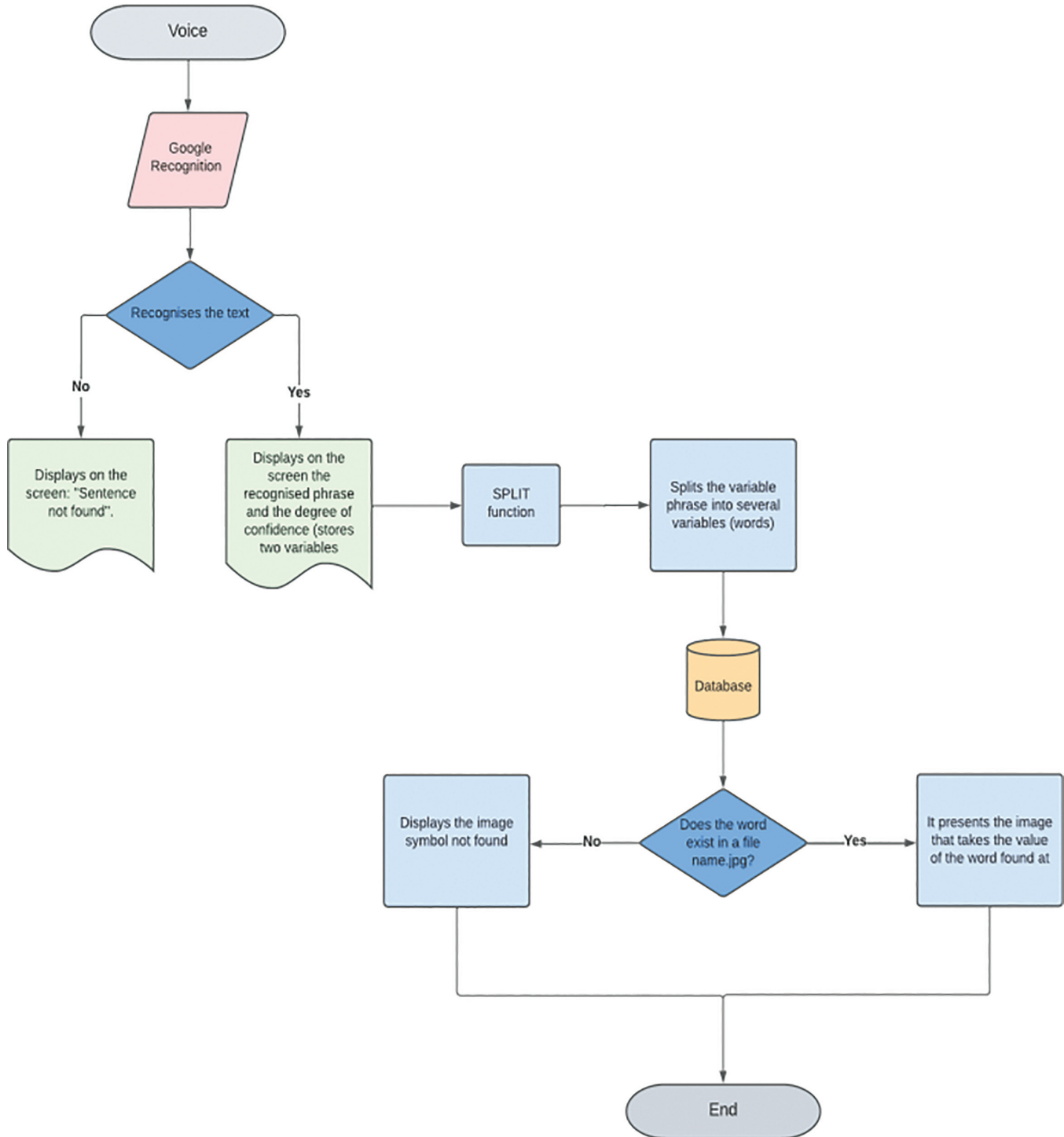
Figure 1. Flowchart of the developed automatic translator.
