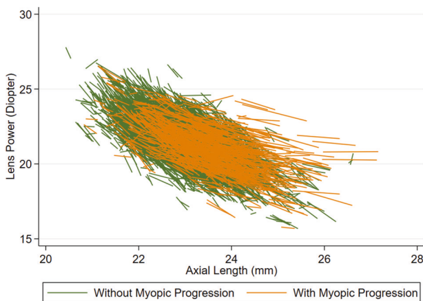
Fig. 2 Three-year changes of lens power by axial length at baseline according to the myopic progression (Spherical Equivalent progression <math>< 0.5</math> diopter). Each line represents individual changes from the baseline to follow-up Phases.
