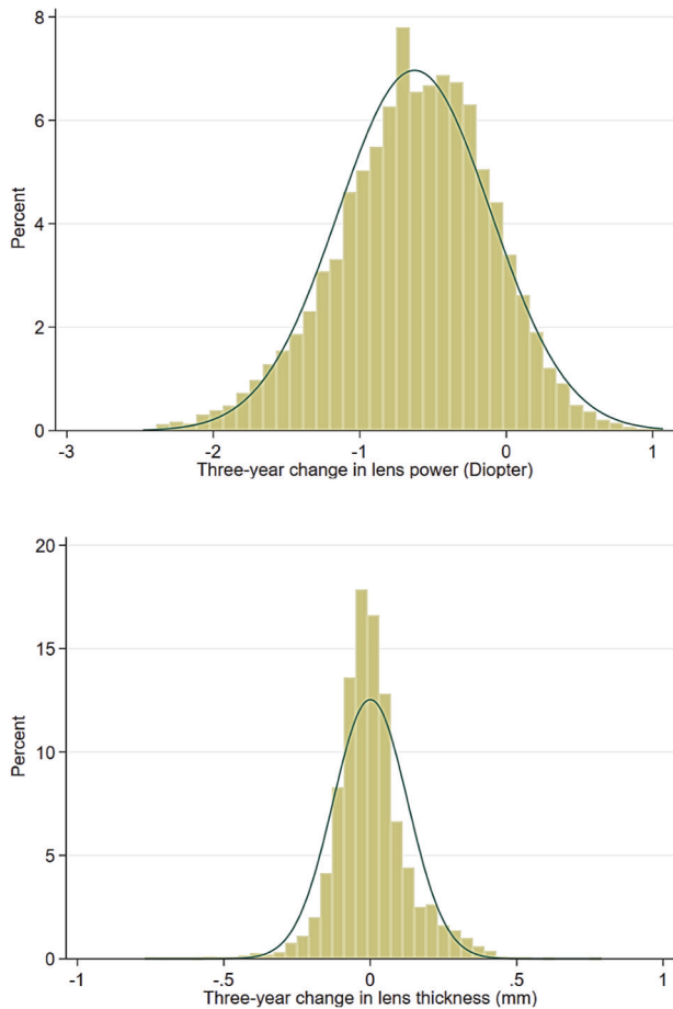
Fig. 1 The distribution of the three-year change in crystalline lens power and thickness. Histograms bars display the percent of individuals in each category and dark lines represent normal distribution curves.
