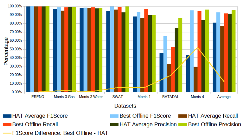
Figure 10. Comparison of best offline algorithm and online reference (HAT) in terms of F1-score, recall, and precision for all datasets.
