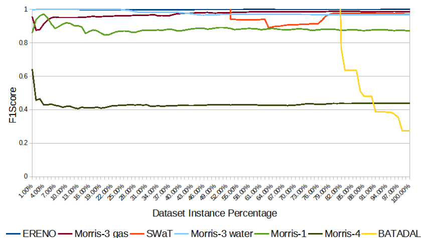
Figure 11. HAT F1-score of all datasets.
