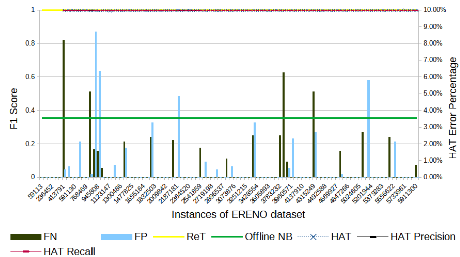
Figure 5. ERENO's F1-score evolution through the samples; attacks are distributed throughout.
