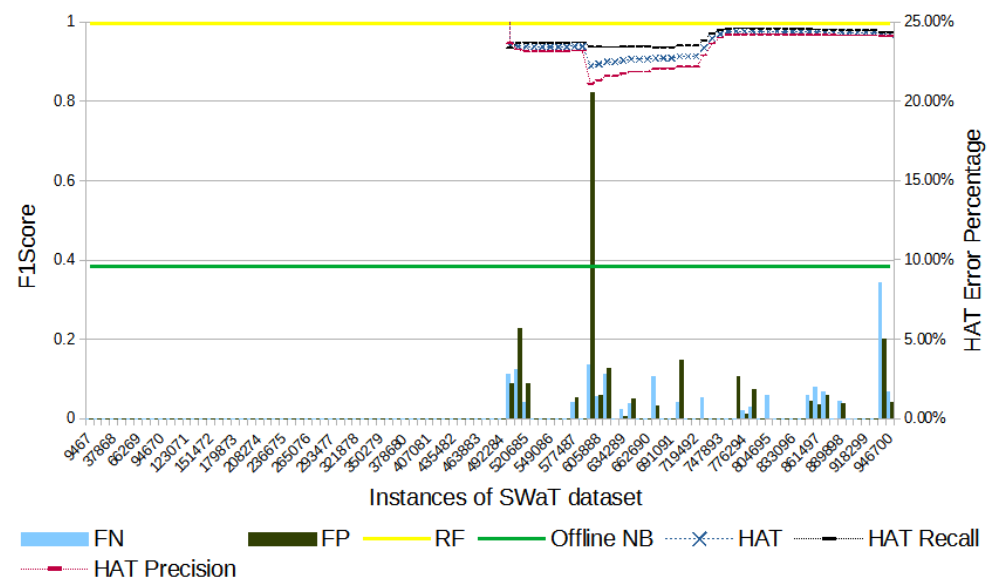
Figure 3. SWaT's F1-score evolution through the samples. The metrics of F1-score, recall, and precision appear only after attacks start, that is, only after sample 492,284.
