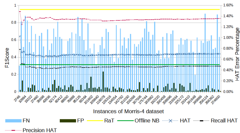
Figure 9. Morris-4's F1-score evolution through the samples.
