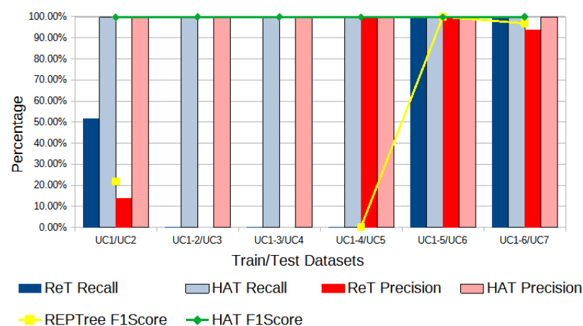
Figure 13. ERENO: cumulative F1-score; best offline (RepTree) and online (HAT) classifiers.
