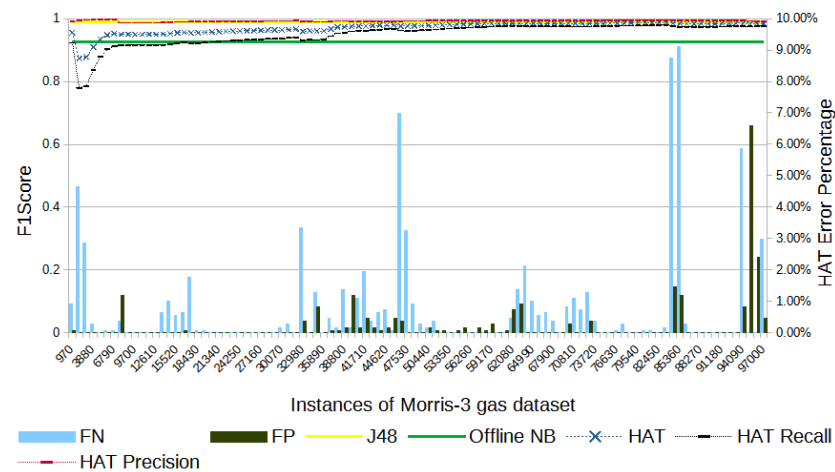
Figure 7. Morris-3 gas's F1-score evolution through the samples.
