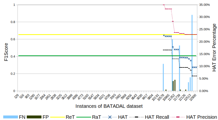
Figure 4. BATADAL's F1-score evolution through the samples. The metrics of F1-score, recall, and precision appear only after attacks start, that is, only after sample 10,578.
