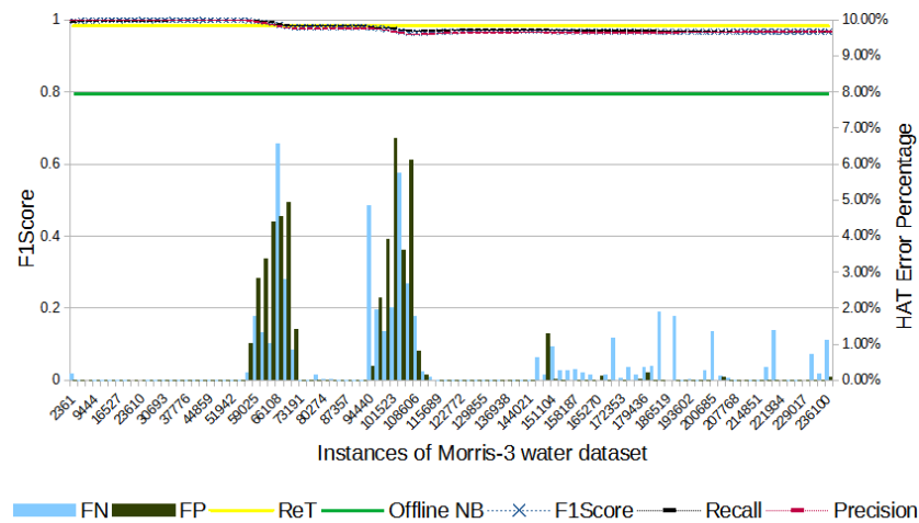
Figure 8. Morris-3 water's F1-score evolution through the samples.
