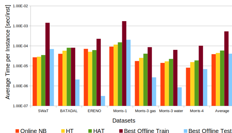
Figure 12. Offline and online classifiers' average run time per instance.
