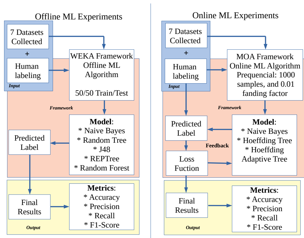
Figure 2. Methodology used in our evaluation of offline and online ML methods.
