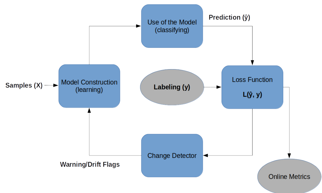
Figure 1. Outline of the online ML with prediction loss function and change detector.
