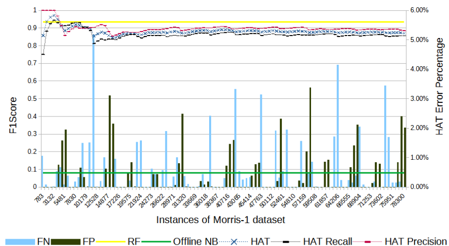
Figure 6. Morris-1's F1-score evolution through the samples; attacks are distributed throughout.
