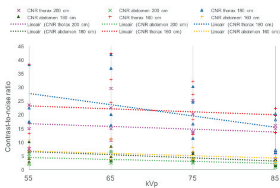
Figure 4: Influence of beam energy (kVp) and source-to-image distance (SID) on contrast-to-noise ratio (CNR) in the thorax and abdominal areas.
