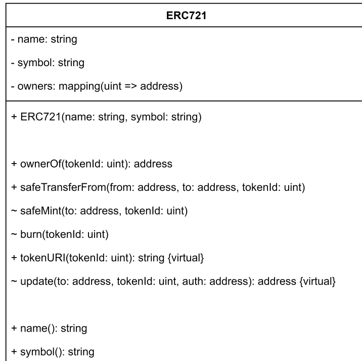
Figure 4.17: ERC721 UML (relevant methods)
