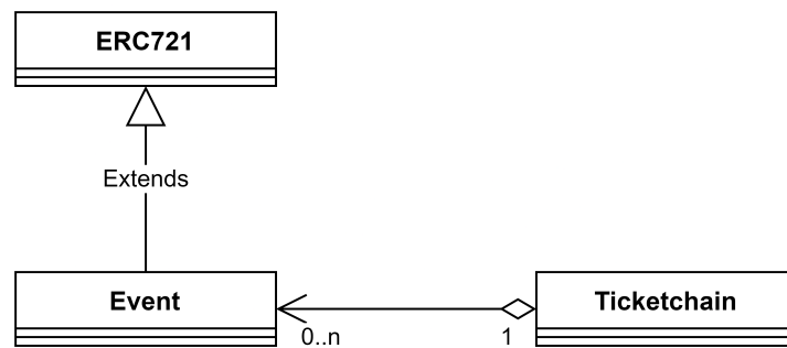
Figure 4.15: System UML (simplified)
