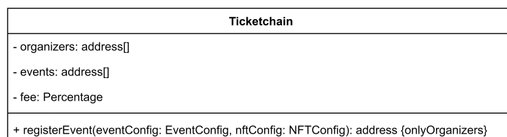
Figure 4.16: Ticketchain UML (relevant methods)
