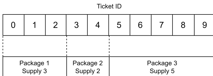
Figure 4.21: Package logic
