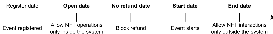
Figure 4.18: Event lifecycle
