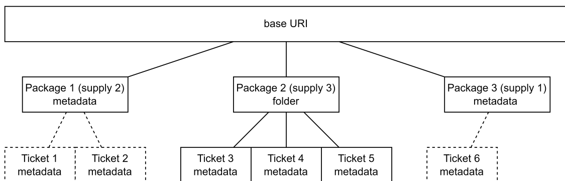
Figure 4.22: Metadata storage
