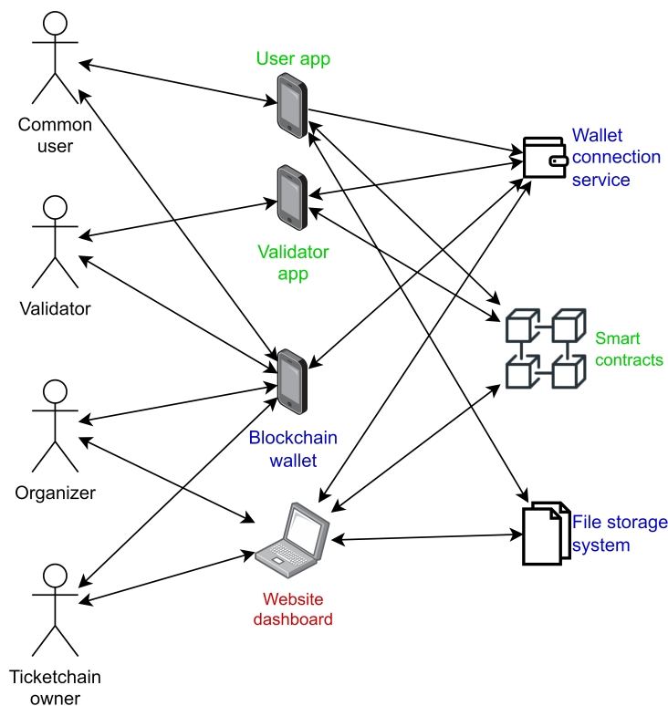
Figure 3.5: System Architecture
