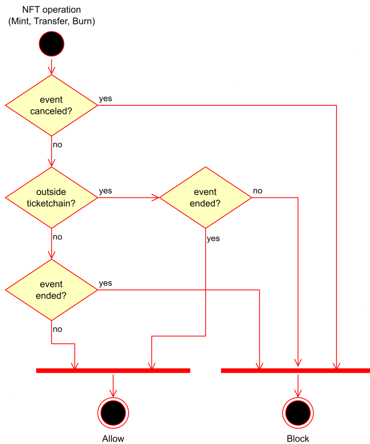
Figure 4.20: NFT flowchart
