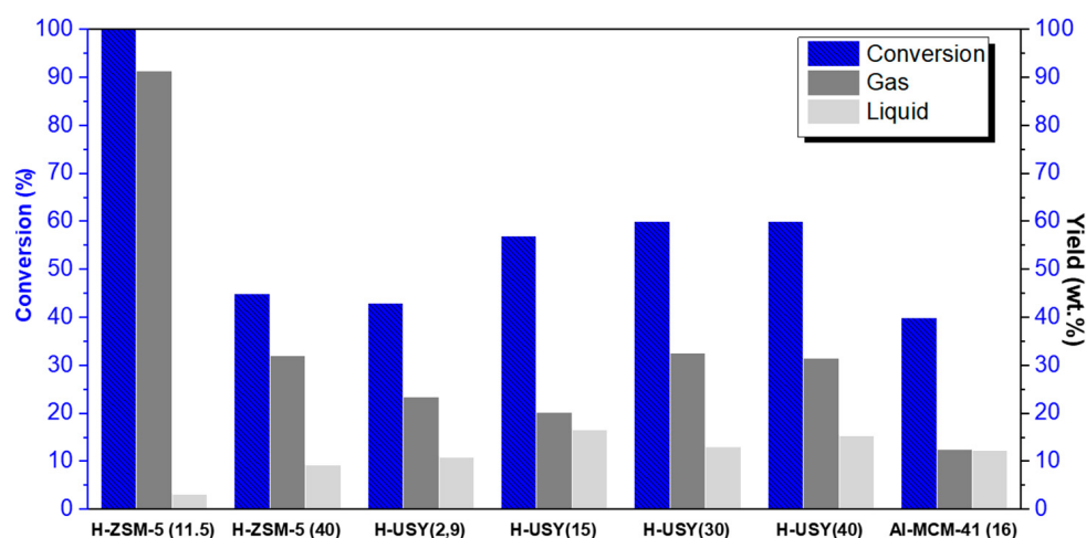
Figure 2. Yields in gas and liquid products obtained from the hydrocracking of HDPE over H-ZSM5 and H-USY with distinct Si/Al ratios and Al-MCM-41 (16) ( T = 300 °C, t = 60 min, P_{\text{H}_2\text{i}} = 20 bar, and HDPE/catalyst mass ratio= 8/2).
