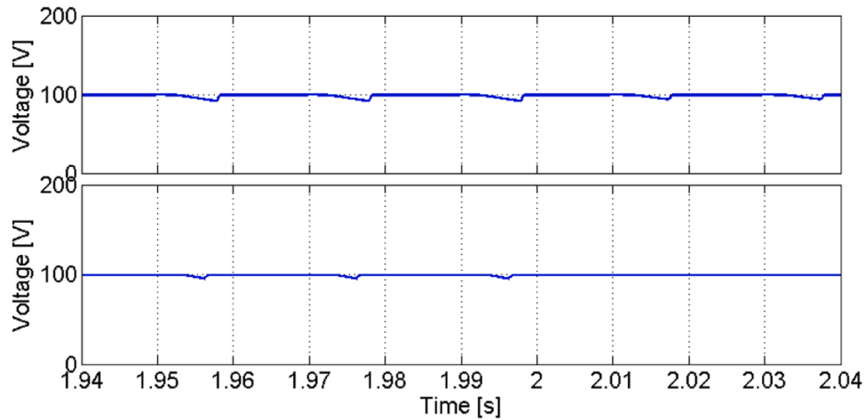
Fig. 11. Simulation result of the capacitor voltages ( V_{C11}(\text{up}) and V_{C12}(\text{down}) ) of the proposed nine-level inverter. This result was obtained for a change in the modulation index from m_a = 0.93 to m_a = 0.66 .
