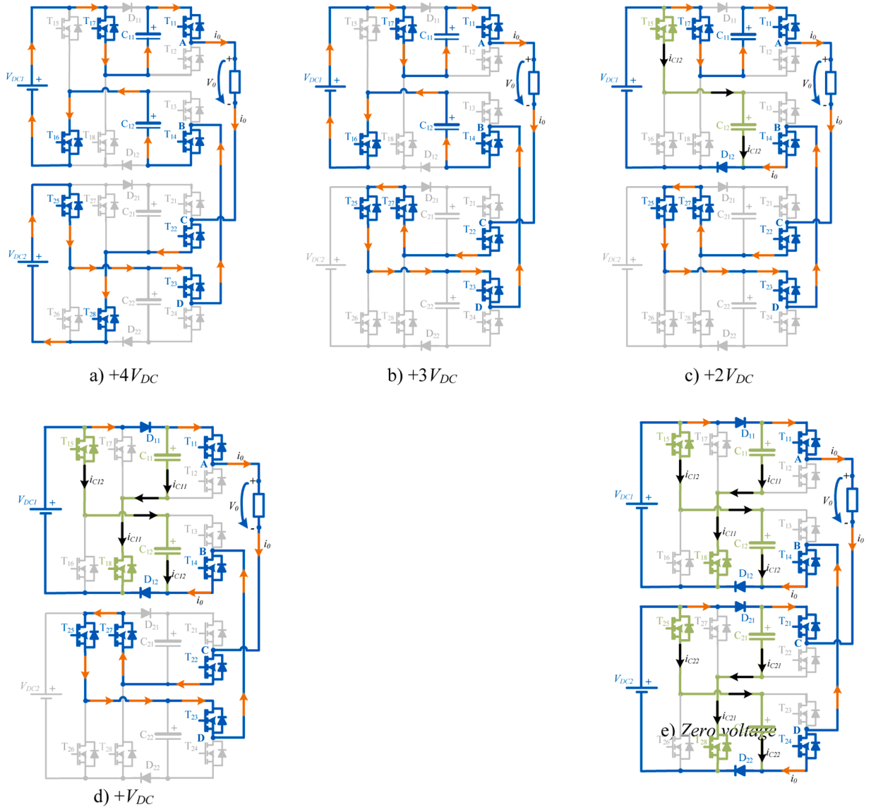
Fig. 2. Operation modes associated to each positive voltage levels associated to the proposed converter.
