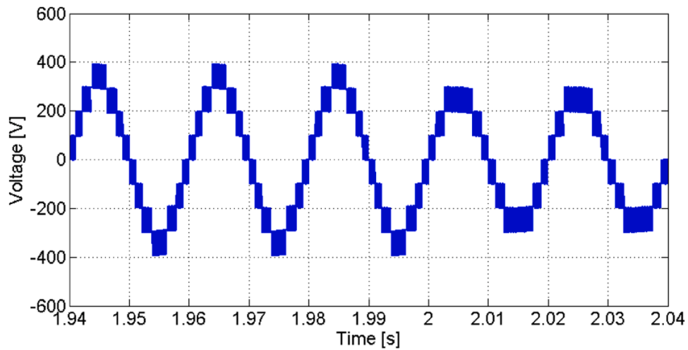
Fig. 10. Simulation result of the output voltage V_o of the proposed nine-level inverter. This result was obtained for a change in the modulation index from m_a = 0.93 to m_a = 0.66 .
