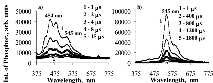
Figure 1: Laser induced room temperature phosphorescence emission spectra from air equilibrated samples of BZP/tri- O -propyl- p-tert -butylcalix[4]arene inclusion complex (molar ratio 1:2.5). a) 500 ns gate width. b) 20 ms gate width.
