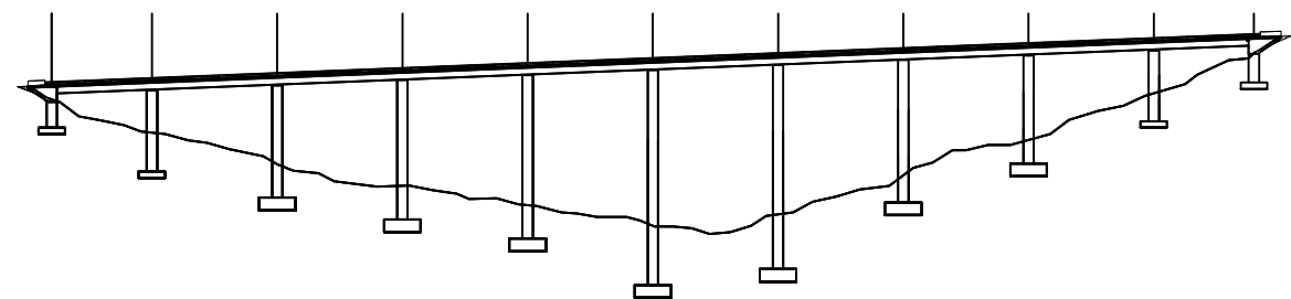
PHASE 11 - CONSTRUCTION OF TENTH SECTION AND FINISHING
