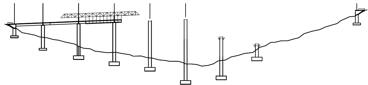
PHASE 4 - CONSTRUCTION OF THIRD SECTION
