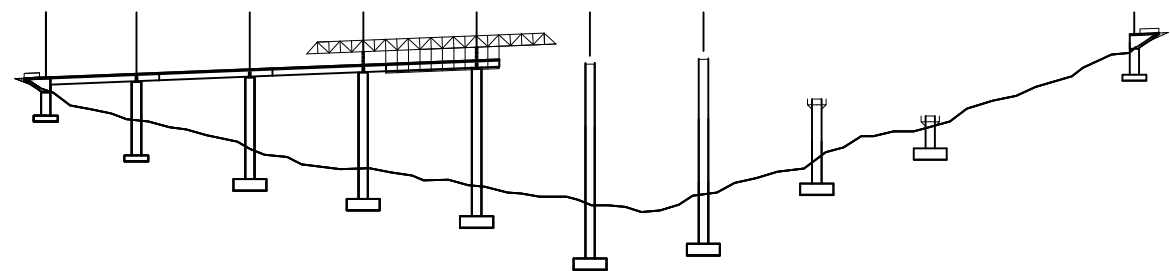
PHASE 5 - CONSTRUCTION OF FOURTH SECTION
