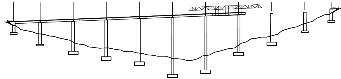
PHASE 8 - CONSTRUCTION OF SEVENTH SECTION
