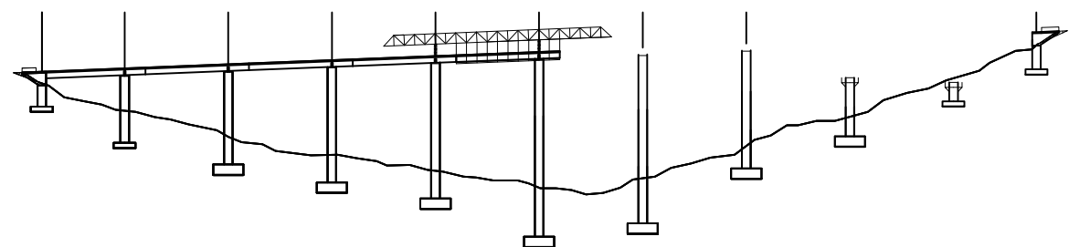
PHASE 6 - CONSTRUCTION OF FIFTH SECTION
