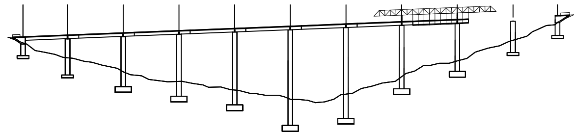
PHASE 9 - CONSTRUCTION OF EIGHTH SECTION
