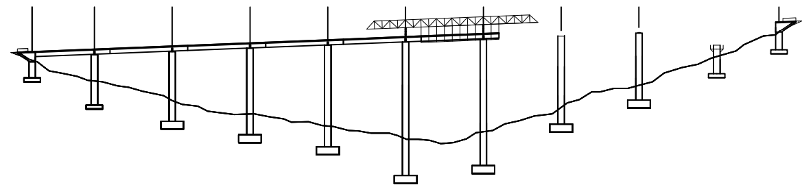
PHASE 7 - CONSTRUCTION OF SIXTH SECTION
