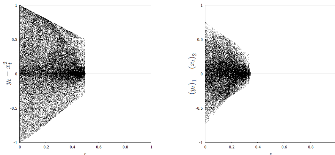
Figure 1. Graphs of the post-transient iterates y_t - R(x_t) as a function of c for an unidirectional coupling with G_2 = -g . At the left, we consider that f is the logistic map and R(u) = u^2 . At the right, we consider that f is the Hénon map and R(u_1, u_2) = (u_2, u_1) .
