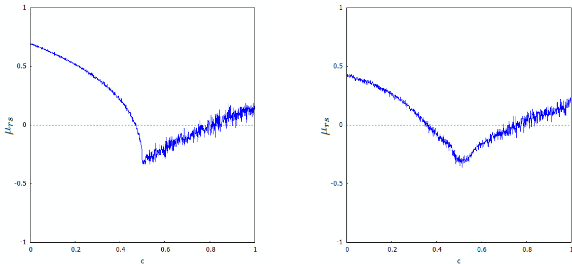
Figure 4. Graphs of \mu_{rs} as a function of c for an unidirectional coupling. At the left, we consider that f is the logistic map, R(u) = u^2 and G_2(u) = -g^2(u) . At the right, we consider that f is the Hénon map, R(u_1, u_2) = (u_2, u_1) and G_2(u_1, u_2) = (-g_1^2(u_1, u_2), -g_2^2(u_1, u_2)) .
