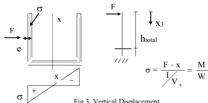
Fig 3. Vertical Displacement
