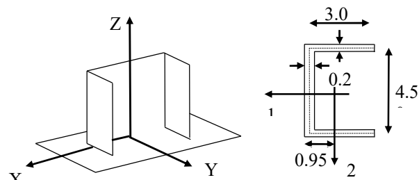
U Section
