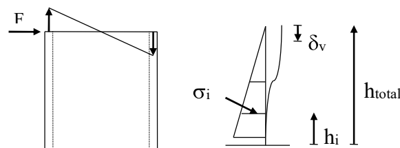
Fig 3. Vertical Displacement
