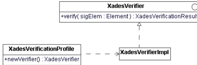
Figure 5.10: Verification profile and signature verifier
