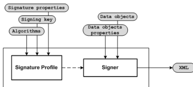
Figure 4.1: Signature production model
