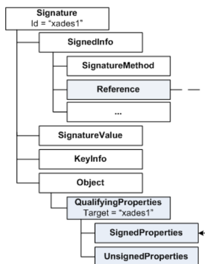
Figure 2.4: XAdES signature structure
