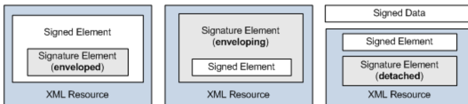
Figure 2.2: Different types of signatures
