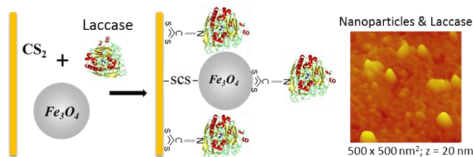
Figure 1 - Schematic representation of the one-step method exploited in this work and an AFM image of modified electrode with Laccase and \text{Fe}_3\text{O}_4 NPs.
