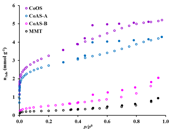
FFFig. 1 Nitrogen adsorption-desorption curves at -196 °C
