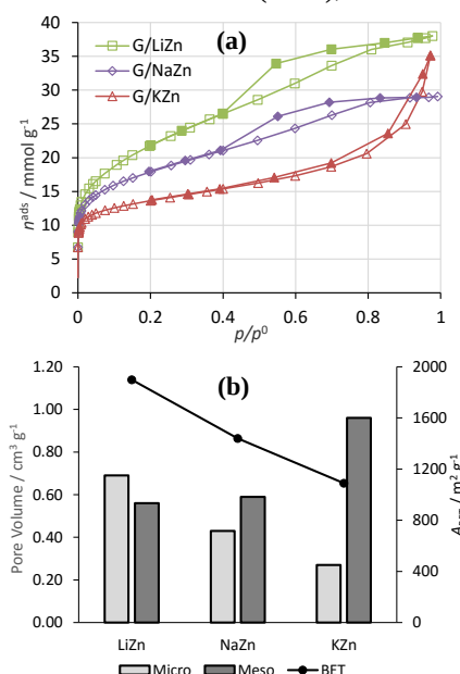
Figure 1. Textural characterization of materials obtained at 800 °C with the mentioned eutectic mixtures (a) N 2 isotherms; (b) textural parameters (bars: volumes; line: A_{\text{BET}} ).
