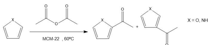
Figure 1. General scheme for the acylation of heteroaromatic compounds.
