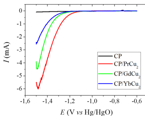
Figure 1. Linear voltammograms recorded for the different electrodes under study at room temperature. Sweep rate of 1 mVs -1 .
