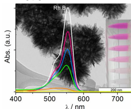
Figure 1. BiOCl-Bi 2 S 3 TEM image and its photocatalytic performance for RhB degradation under UV-vis light irradiation.
