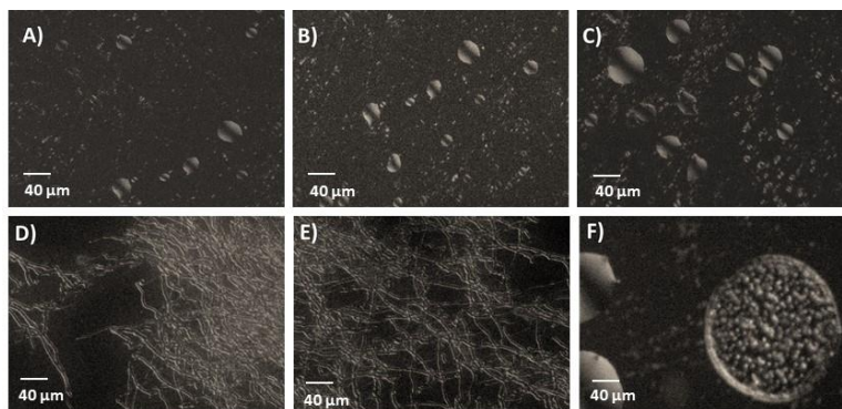
Figure 1. Transmission microscopy images for N. crassa WT and slime cells at different phases of growth. WT cells in MMV at 5 h (A) and 12 h (D) of growth; WT cells in SeM at 5 h (B) and 12 h (E) of growth; slime cells at 5 h (C) and 12 h (F) growth), with a magnification of 100 \times .
