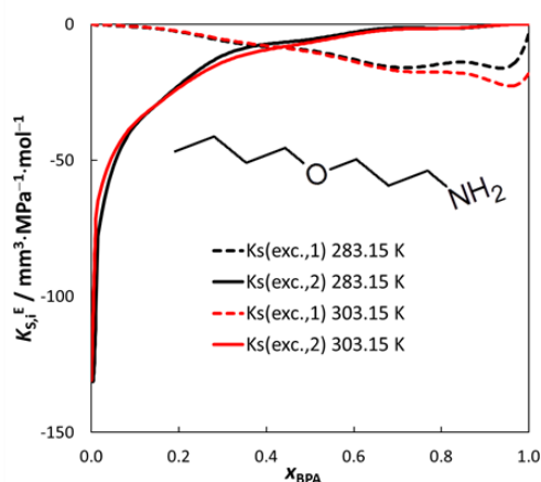
Figure 1 Excess partial molar isentropic compressions
