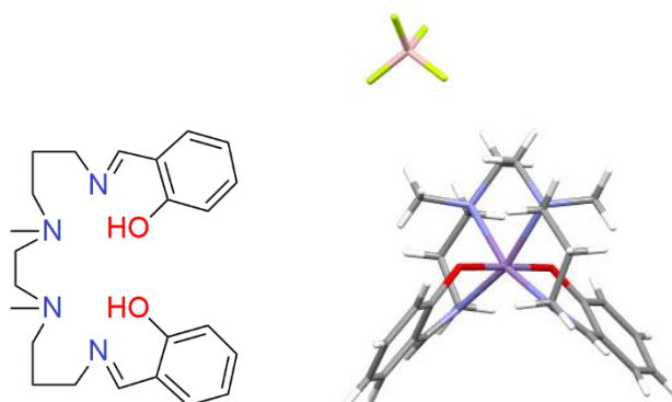
Figure 1 – Schiff-base ligand used in this study (left) and single crystal X-ray structure of the Mn(III) BF_4^- salt (right).
