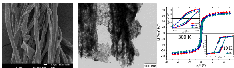
Figure 1. SEM image of gauze (left); TEM image of CoFe 2 O 4 nanoparticles obtained after gauze calcination (middle); magnetization results of all samples obtained after template calcination (right).
