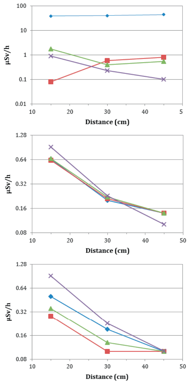
Figure 4 How the dose rate, detected by, a) the RadioactivityCounter, b) Pocket Geiger Type6 and c) Smart Geiger changes with distance, all with use of the three smartphones HTC(blue), Samsung(green), Sony(red) and the calculated dose rate(purple).
