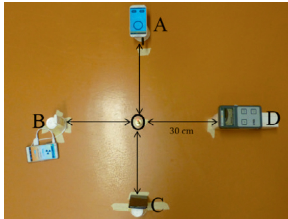
Figure 2 Setup of measurement with Constant exposure, different sources. The devices are A: Smart Geiger, B: Pocket Geiger Type6, C: RadioactivityCounter and D: Messbereich FH40F2. All devices were 30 cm from point O where the different radioactive sources were placed.
