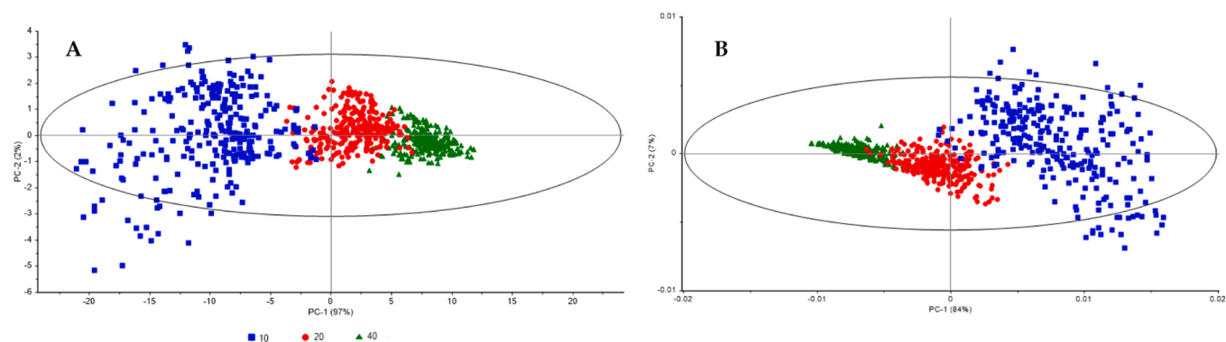
Fig 4. PCA of baseline corrected spectra (A), or the second derivative spectra (B) of non-centrifuged whole blood samples diluted with NaCl solution at 1/10 (blue), 1/20 (red) and 1/40 (green). The Hotelling's T^2 ellipse is at 1 % significance.
