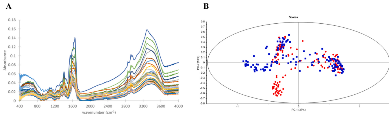
Fig 2. Example of spectra without pre-processing of methanol-based extracts from defrosted whole blood (A) and PCA based on normalised second derivative spectra of exposed (blue) in relation to non-exposed volunteers (red) (B).
