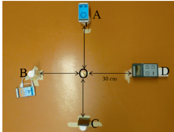
Figure 2 Setup of measurement with Constant exposure, different sources. The devices are A: Smart Geiger, B: Pocket Geiger Type6, C: RadioactivityCounter and D: Messbereich FH40F2. All devices were 30 cm from point O where the different radioactive sources were placed.
