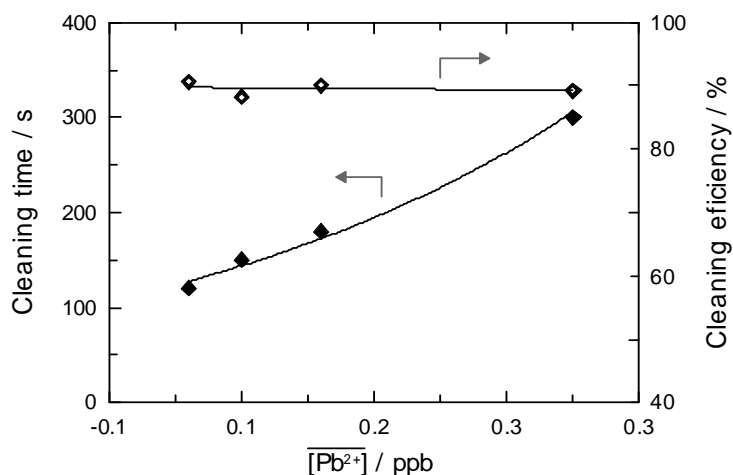
Fig. 3 - Crossing data between average Pb^{2+} concentration, mercury film cleaning time and mercury film cleaning efficiency.
