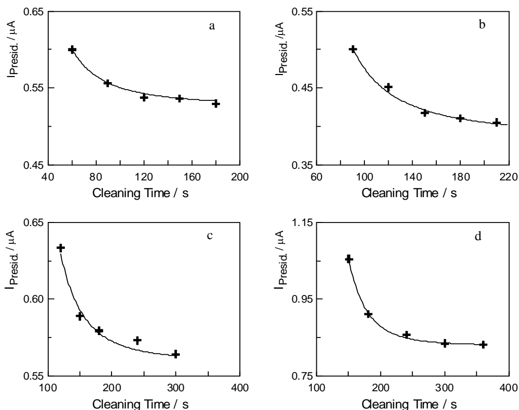
Fig. 1 - I_{\text{resid.}} for \text{Pb}^{2+} vs. Mercury film cleaning time. Concentrations under study a: 0.020 ppb, b: 0.080 ppb, c: 0.200 ppb and d: 0.600 ppb.
