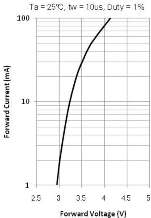
Forward Current – Forward Voltage
