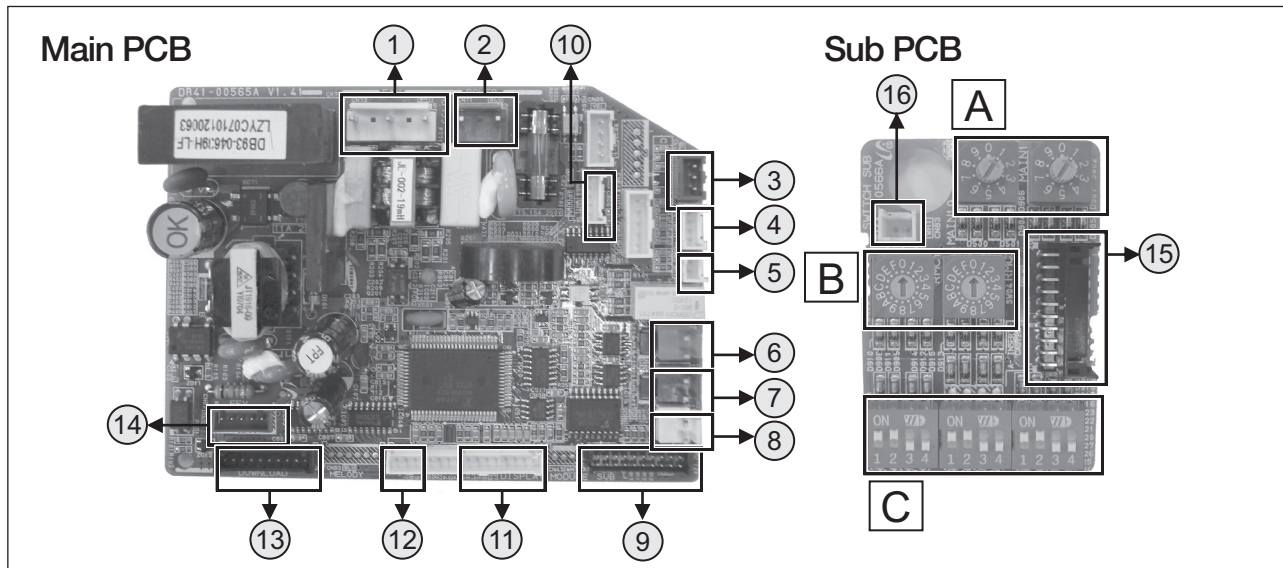
Main PCB
