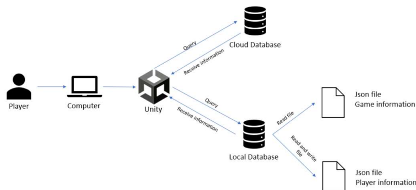
Figure 1. Diagram of the architecture of the proposed solution.
