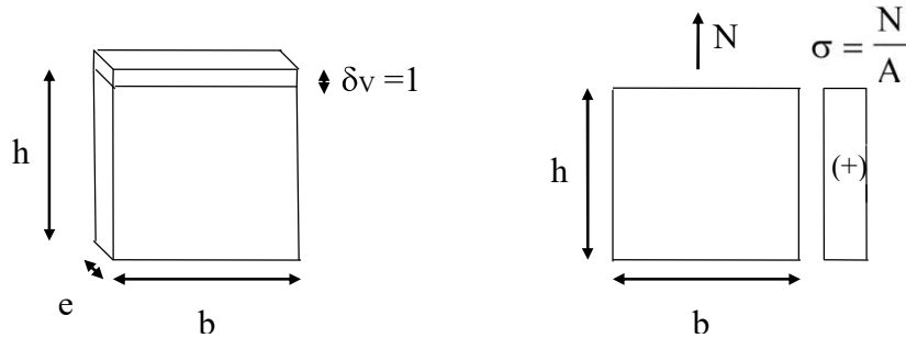
Fig. 1 - Applying a unit vertical displacement to a plate element
