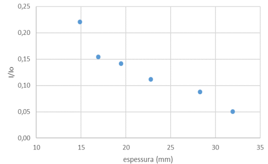
Figure 4: Results of attenuation studies for N-150 radiation quality.
