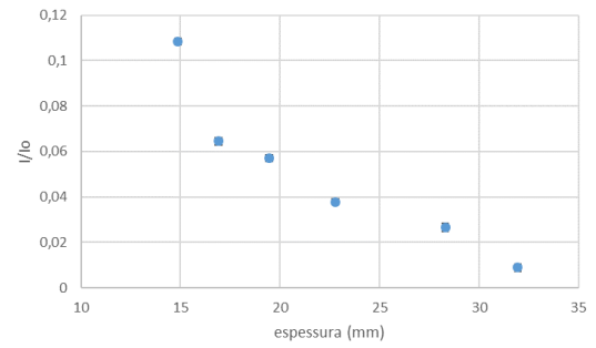
Figure 3: Results of the attenuation studies for the quality of N-120 radiation.
