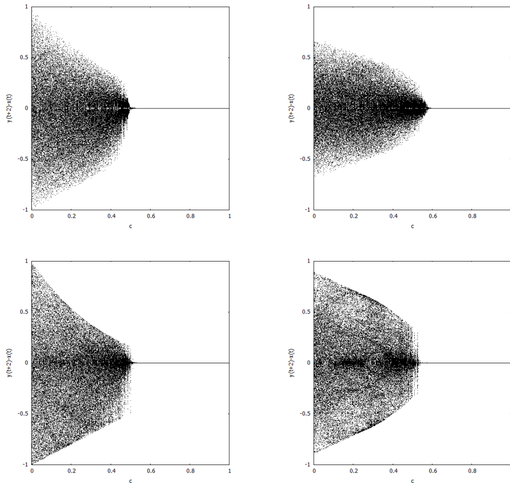
Figure 5: Graphs of the iterates y(t + 2) - x(t) as a function of c for the CPFC of the tent map (at the top left), the logistic map (at the bottom left), the 3-piecewise linear map (at the top right) and the cubic-like map (at the bottom right)
