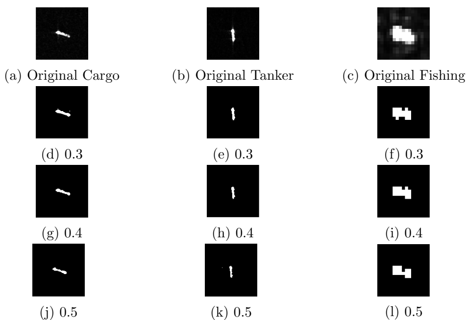
Figure 12: Application of the CFAR algorithm with different thresholds and ship types. The image is organized by: Lines - Different thresholds and Columns - Different ship types.
