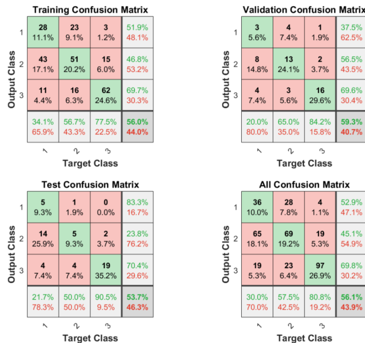
Figure 6: Confusion matrix.
