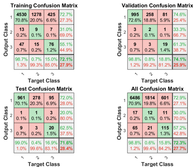
Figure 5: Confusion matrix.
