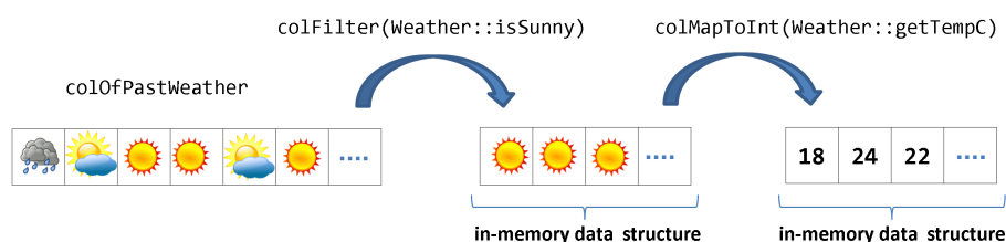
Figure 2.2: In-memory data structures produced by the eager execution of colFilter and colMap .
