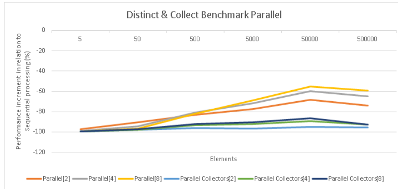
Figure 4.53: Distinct & Collect benchmark results
