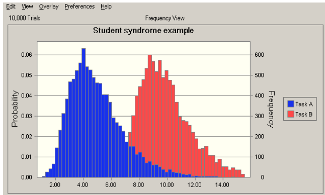
Fig.8-Student Syndrome example.
